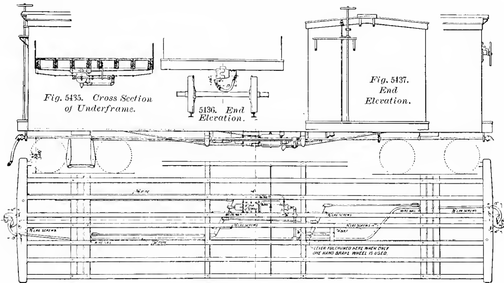
Figs. 5433-31. Elevation and Plan. STANDARD AIR-BRAKE GEAR FOR FREIGHT-CARS.
